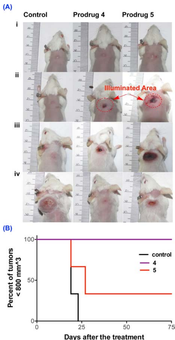
Figure 8. (A) Photographic images of mice (3 mice per group) treated with prodrug (none, 4, or 5 at 2 \mu\text{mol/kg} ) with illumination (690 nm laser, 12 mm diameter circular beam, 100 \text{mW}/\text{cm}^2 , 30 min) 7 h post IV administration of the prodrug: (i) day 0 before illumination, (ii) day 1, (iii) day 6, and (iv) day 15 post-illumination. (B) Kaplan–Meier plot of response to treatment.
