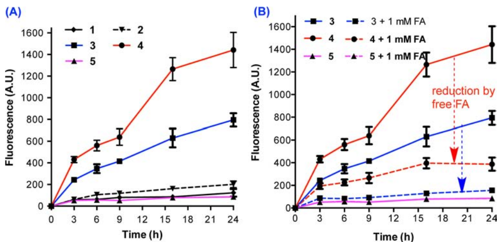
Figure 4. (A) Time-dependent cellular uptake of prodrugs 1–5. Colon 26 cells were incubated with 10 \mu M prodrugs. At various time points, the prodrugs in the cells were quantified by fluorescence emitted from Pc of the prodrugs. (B) Impact of excess free FA on the cellular uptake of the prodrugs. Cells were pretreated (1 h) with 1 mM free FA before the addition of 10 \mu M of prodrugs 3, 4, and 5. The prodrugs in cells were quantified in the same way as in (A). Data are means \pm SD ( n = 3 ).
