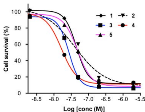
Figure 5. Phototoxicity of prodrugs 1 – 5 against colon 26 cells. Cells were incubated with the prodrugs for 7 h, washed 3 times with PBS, and then illuminated with 690 nm at 5.6 mW/cm 2 for 30 min (10 J/cm 2 ). Cell viability was determined with MTT assay 72 h after the illumination, and expressed as mean percentage \pm SD ( n = 3 ) with respect to untreated control cells. (N.B. SD is not presented here.)
