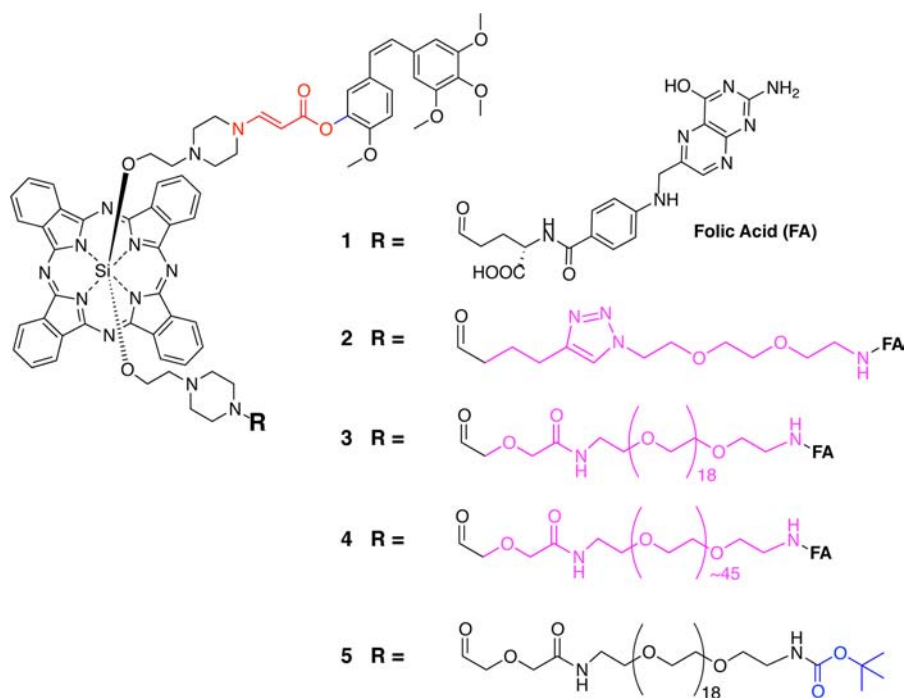
Figure 3. Structures of targeted prodrugs 1–4 and nontargeted prodrug 5.
